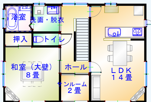
2F PLAN
